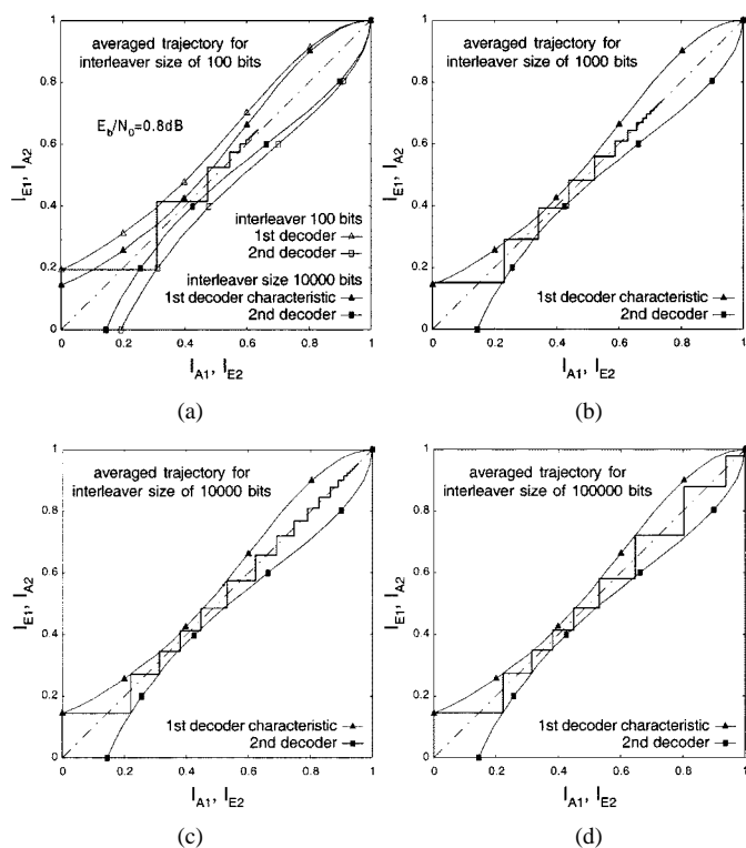
Fig. 8. Averaged decoding trajectories for different interleave lengths; PCC rate 1/2 memory 4, (G_r, G) = (023, 037) ; averaged over 10^8 information bits.
