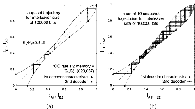
Fig. 7. Transition from snapshot trajectory to averaged trajectory; E_b/N_0 = 0.8 dB; PCC rate 1/2 memory 4, (G_r, G) = (023, 037) ; interleave size 10^5 bits.
